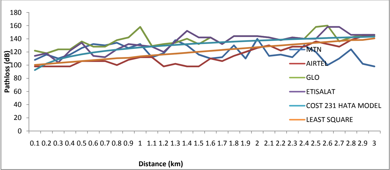
Figure 5: Pathloss (dB) against Distance (km)for MTN, AIRTEL, GLO, ETISALAT, COST 231HATA AND LEAST SQUARE.
