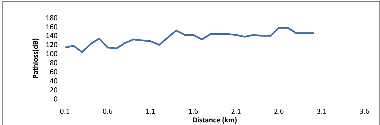
Figure 1: Pathloss (dB) against Distance (km) for ETISALAT network.
