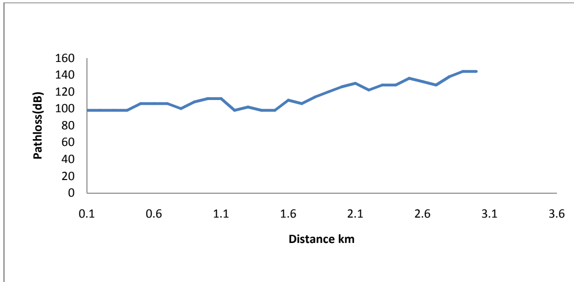
Figure 4: Pathloss (dB) against Distance (km) for AIRTEL network
