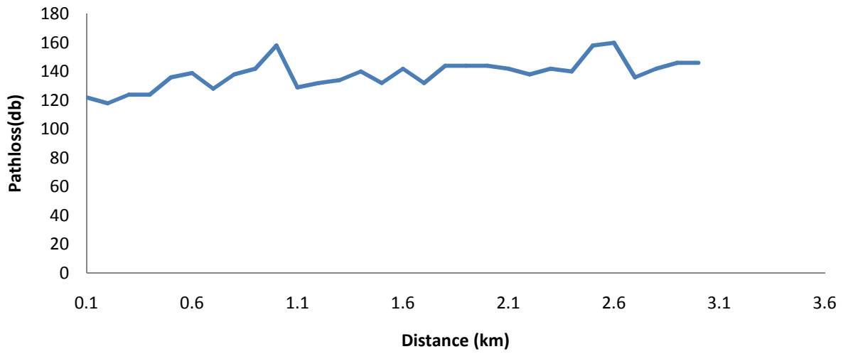
Figure 2: Pathloss (dB) against Distance (km) for GLO network
