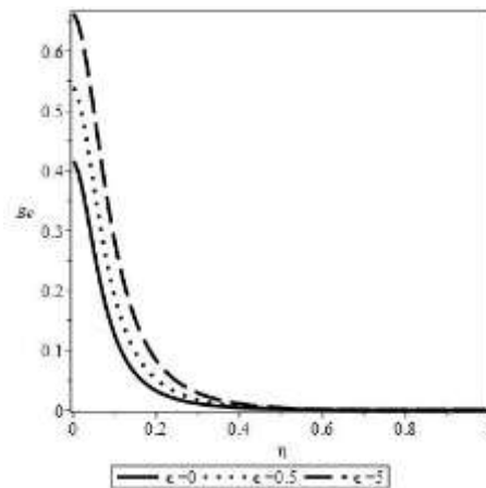
Figure 8: Bejan profile for various values of Biot number
