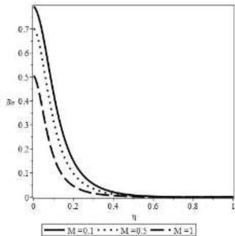
Figure 7: Bejan profile for various values of Brickman number
