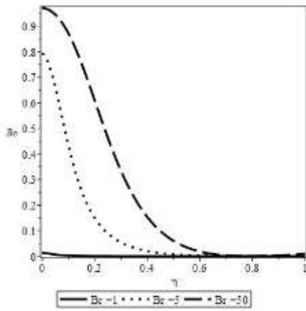
Figure 3: Temperature profile for various values of Biot number
