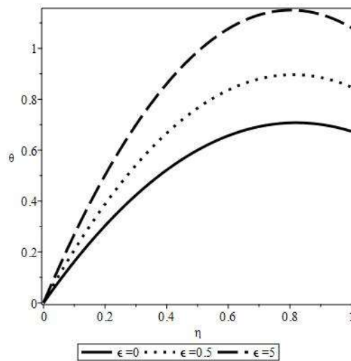
Figure 2: Temperature profile for various values of Thermal conductivity
