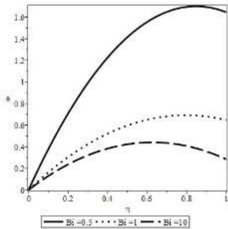
Figure 5: Bejan profile for various values of Magnetic parameter
