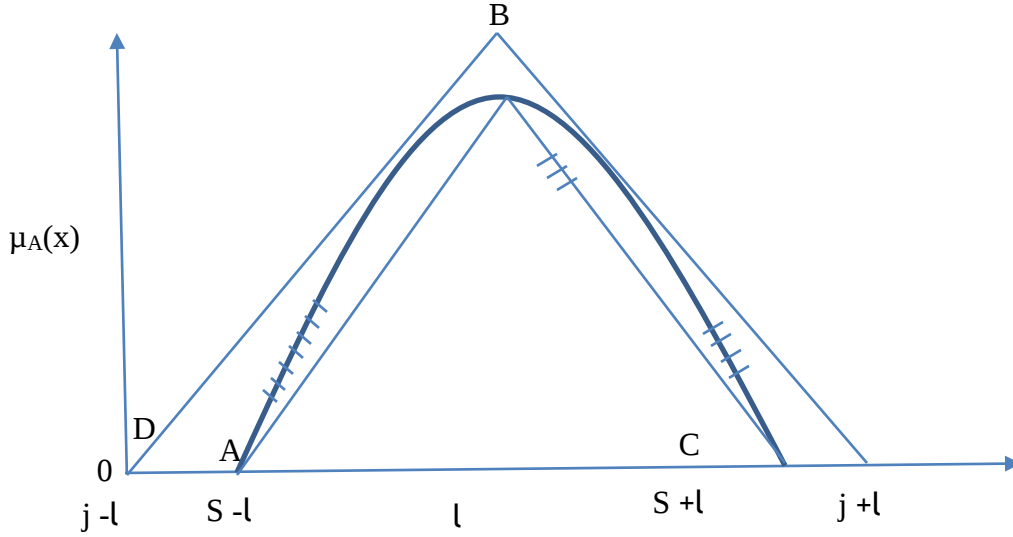
Figure 6: Fuzzy representation for triangular and Semi-circle number
