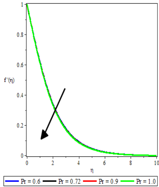
Fig 6: Influence of Pr on velocity profile
