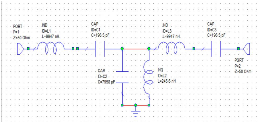
Figure 2: Simulated Circuit Diagram of the Transformed LPF to BPF
