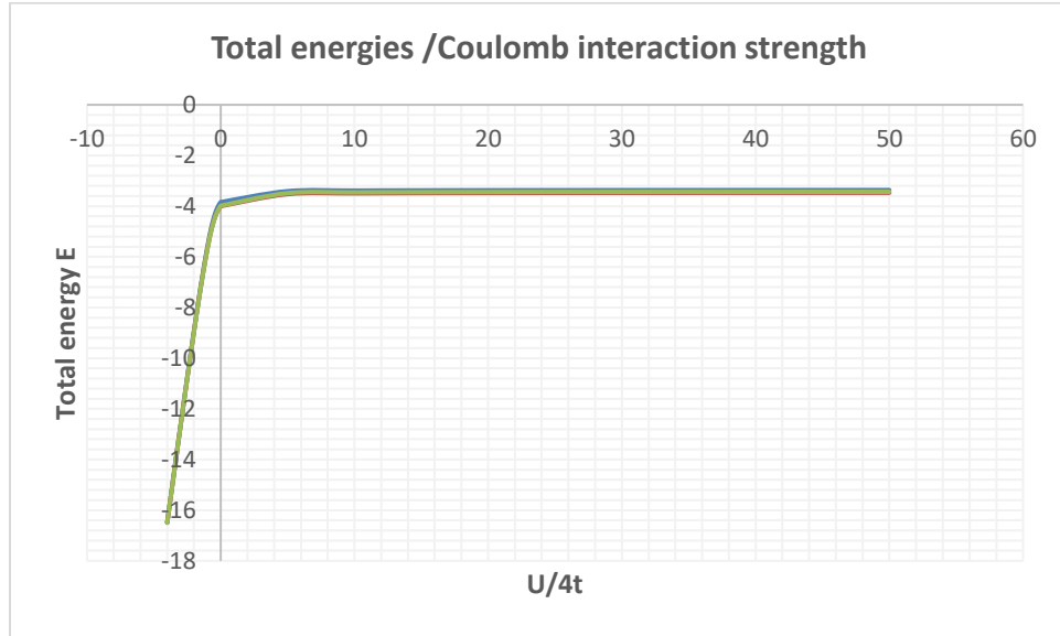
Figure 3.1: Shows the spectrum of the total energies E as a function of the Coulomb interaction strength U/4t for the four types of Hubbard model. This is just the graphical representation of the four model results shown in Table 3.0.
